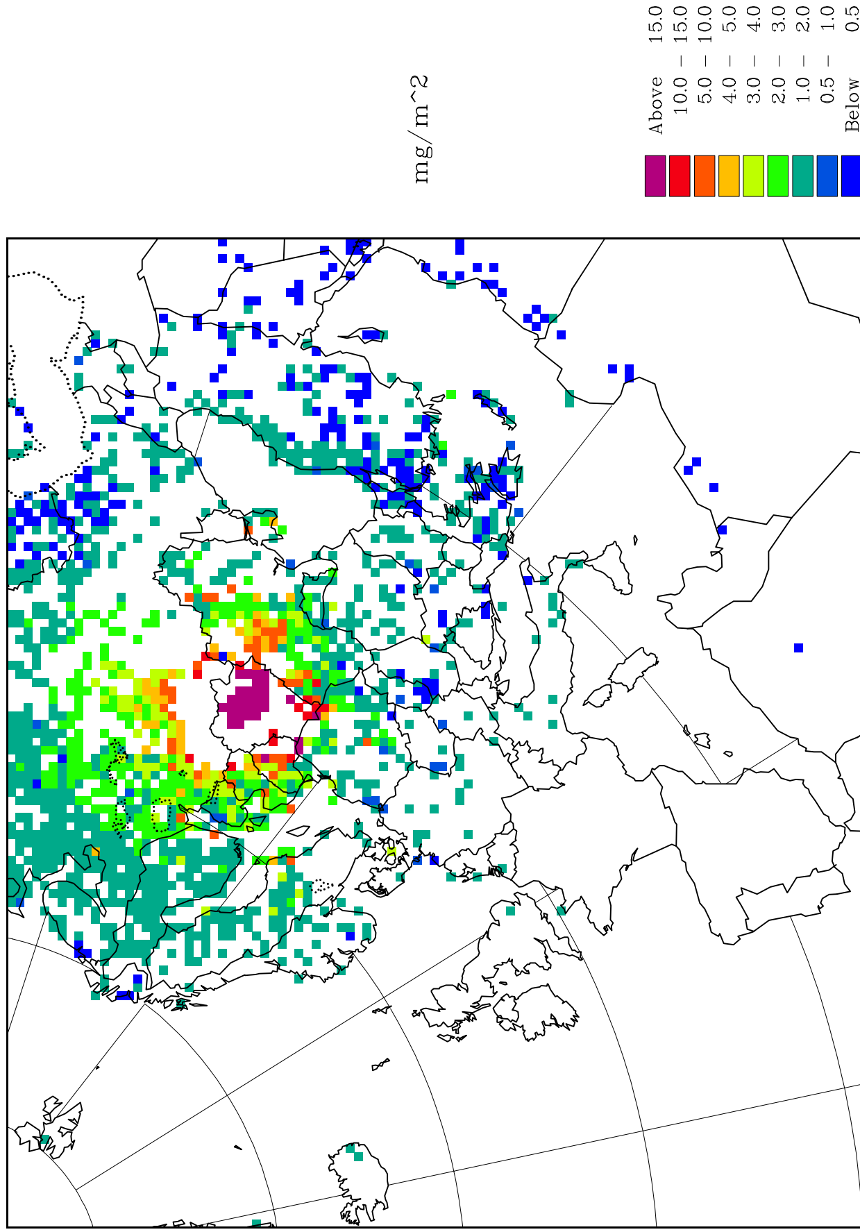
d DepS/d(SOx+NOx+NH3) Seminatural 2000 25% emis. red. from Belarus
