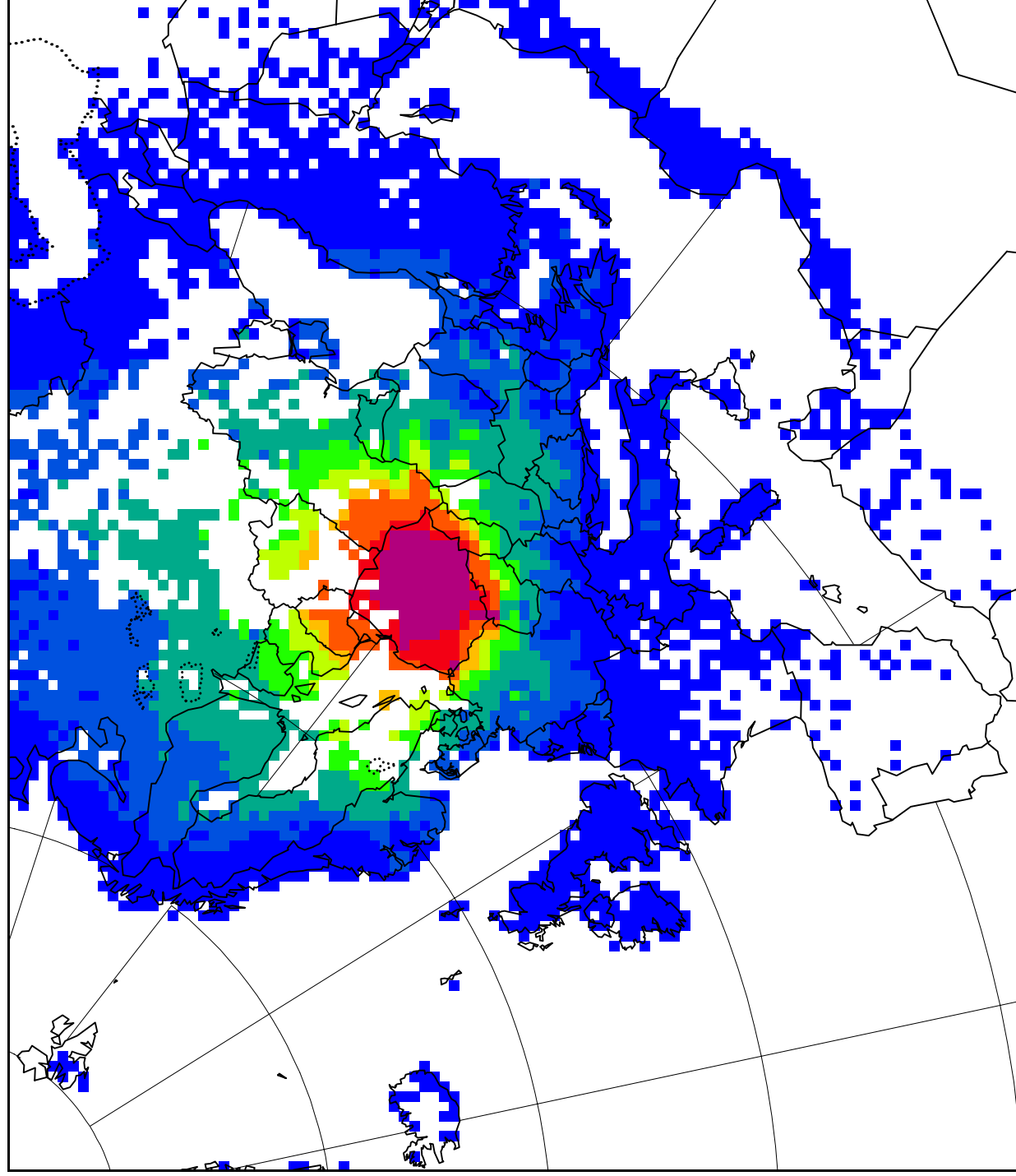
d DepS/d(SOx+NOx+NH3) Seminatural 2000 25% emis. red. from Poland
