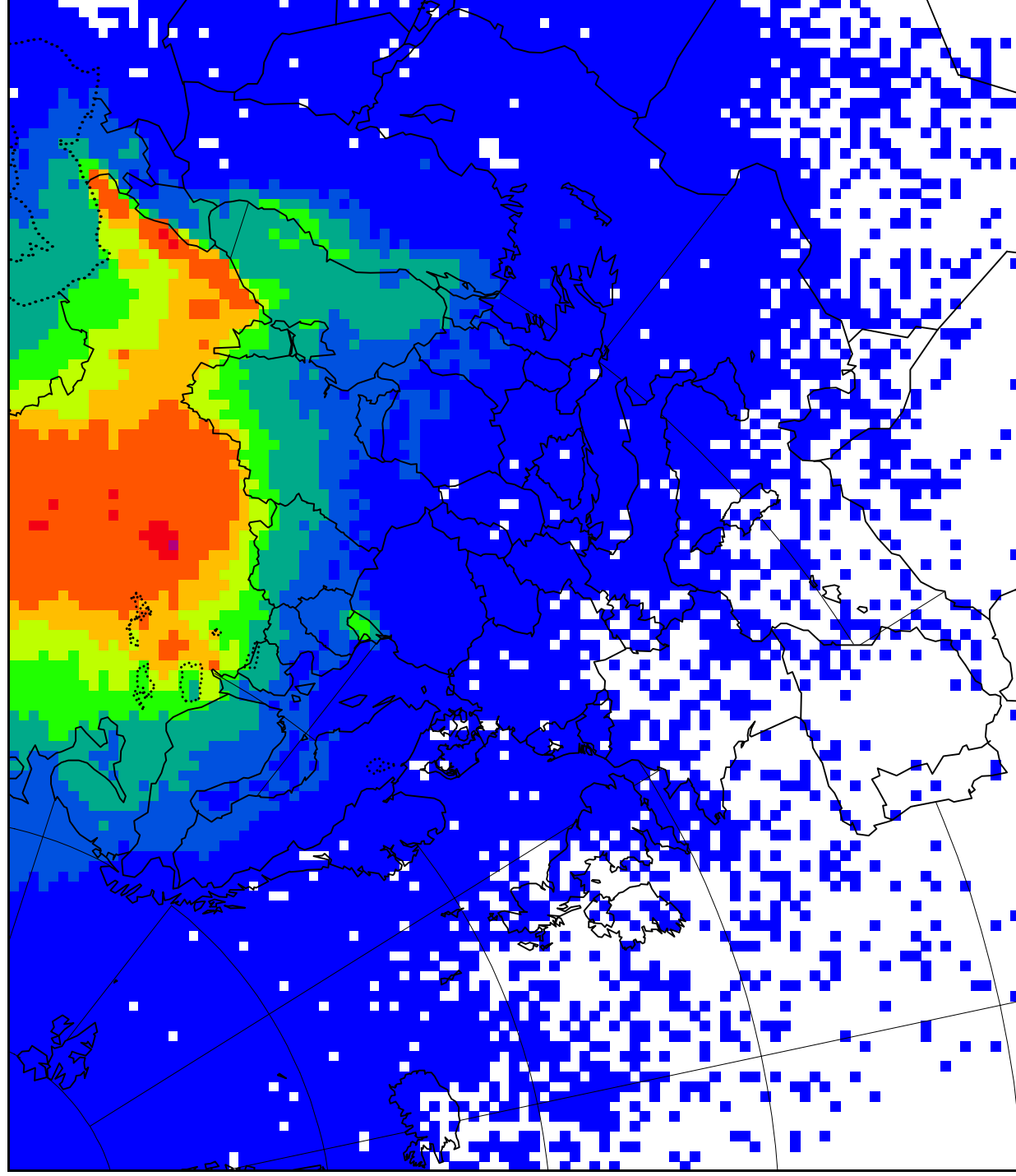
d DepN/d(SOx+NOx+NH3) 2000 25% emis. red. from Russian Federation
